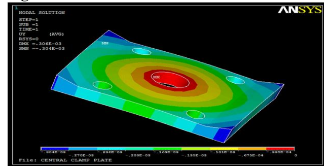
Fig: CENTRAL CLAMP PLATE
