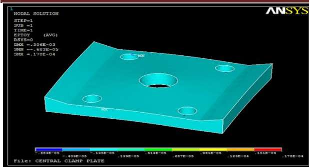
Fig: CENTRAL CLAMP PLATE
